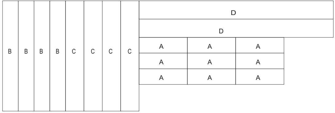
Direction of grain
